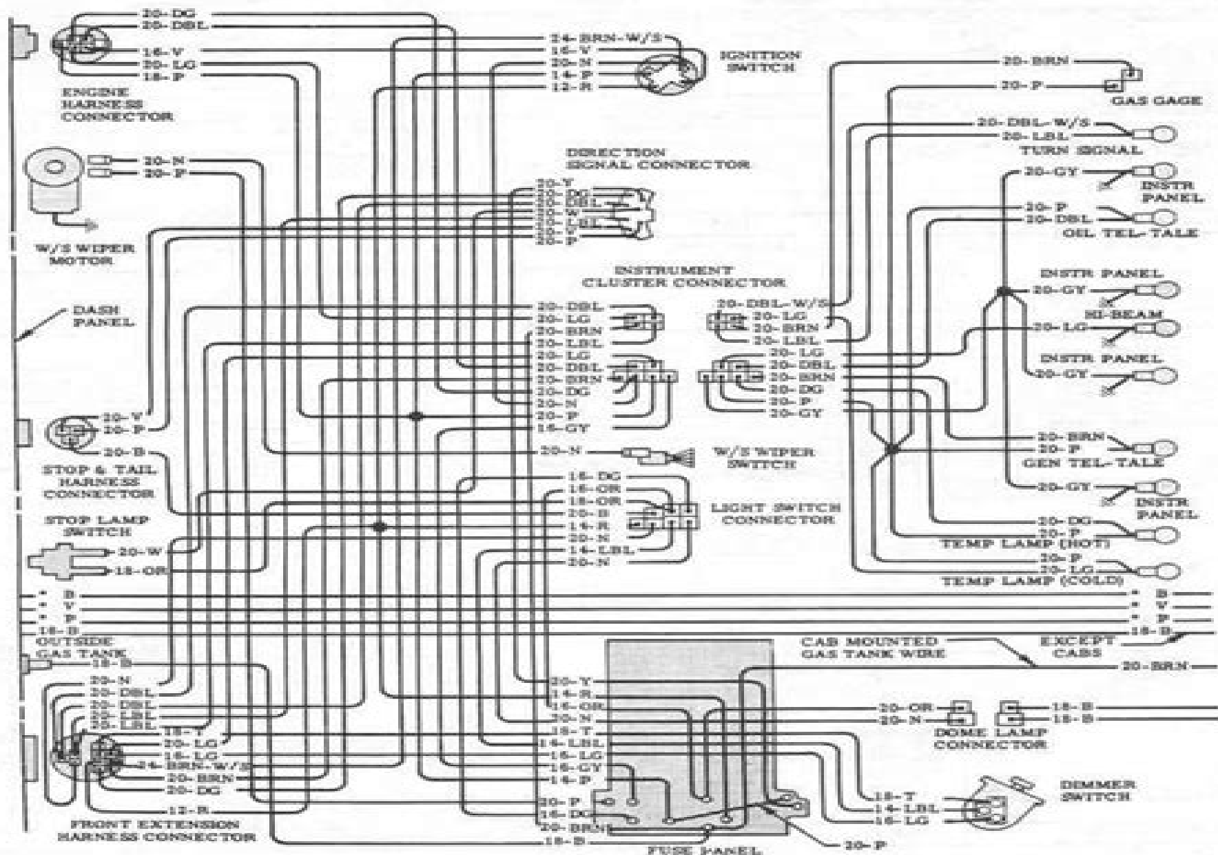
Instrument Panel and Cab—Models: C-K10-20, C-30 (Except F/F Crew)
