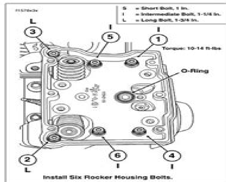
Figure 3-37. Rocker Housing Torque Sequence and Bolt Size (Rear Cylinder Shown)
