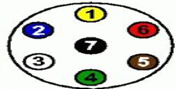
rear of socket, front of plug
