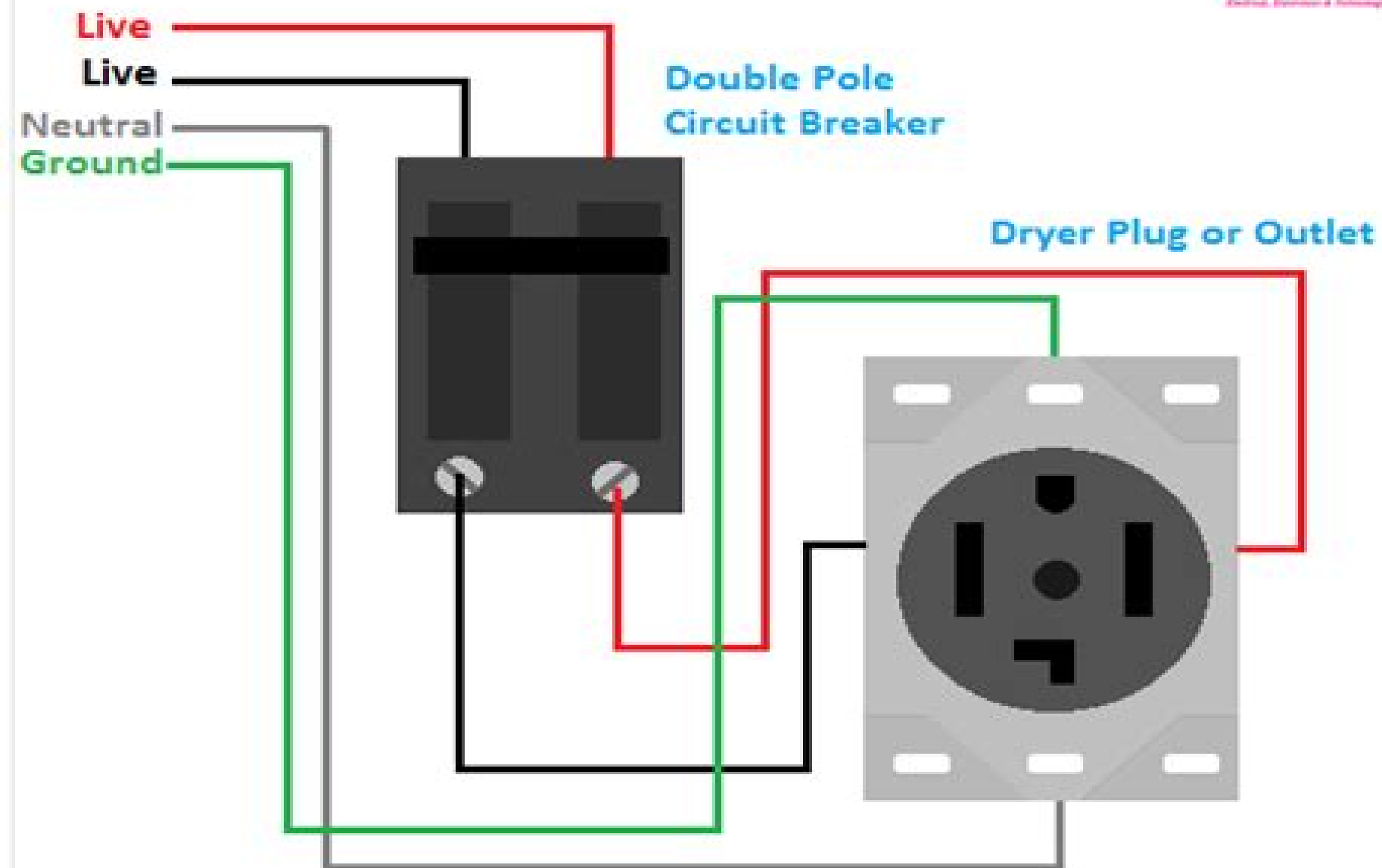
4 Prong Dryer Outlet Wiring Diagram
