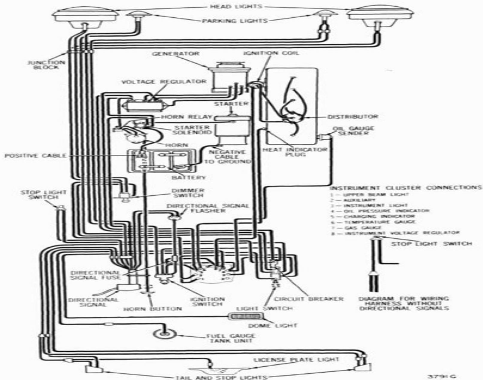
FIG. 156—WIRING DIAGRAM—L6-226 4x4 AND 4x2
