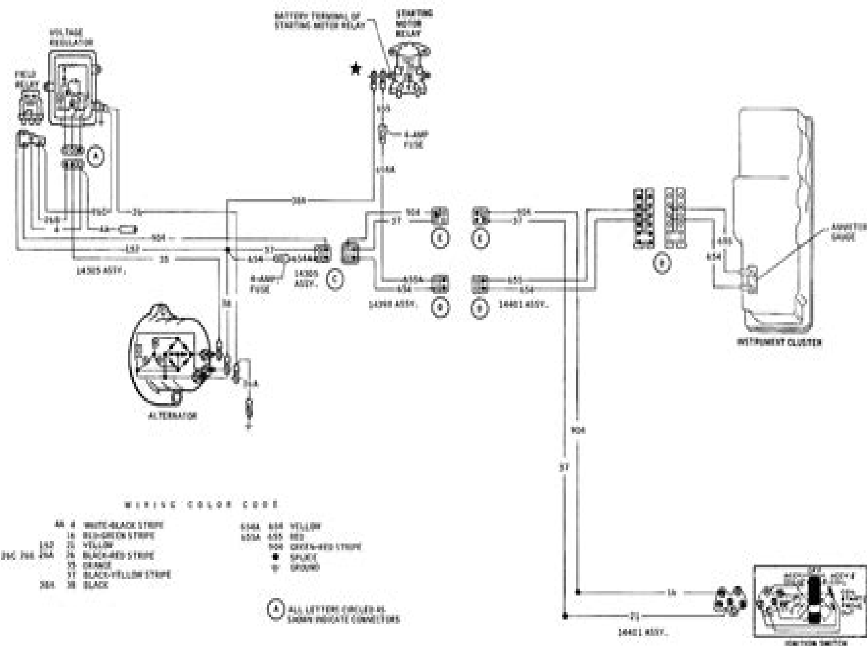
1968 F-100 THRU 750 AND B-500 THRU 750 SERIES TRUCK 65 AMPERE ALTERNATOR
