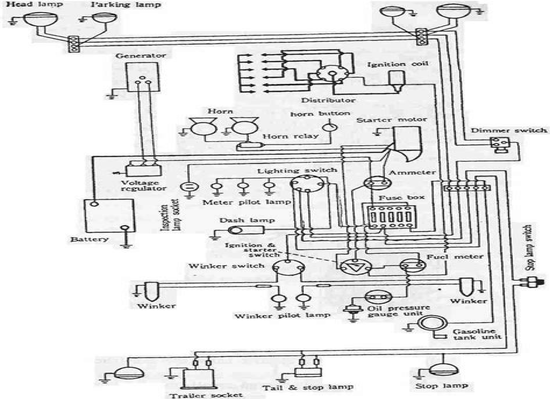
Toyota Model FJ251. Land Cruiser Wiring Diagram
