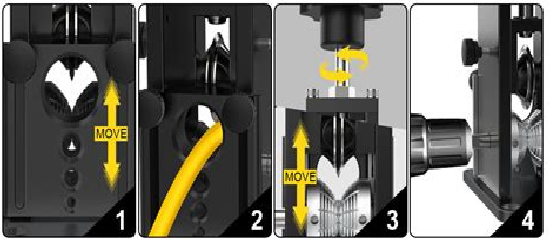
Adjust the feeding hole according to the diameter of the wire
