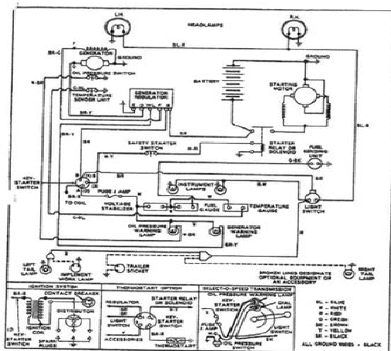
Fig. 160—Wiring diagram for all models with "C" prefix to tractor serial number. Refer to page 2 of this manual for serial number location. For tractors with "A" or "B" prefix to tractor serial number, refer to Fig. 161.
