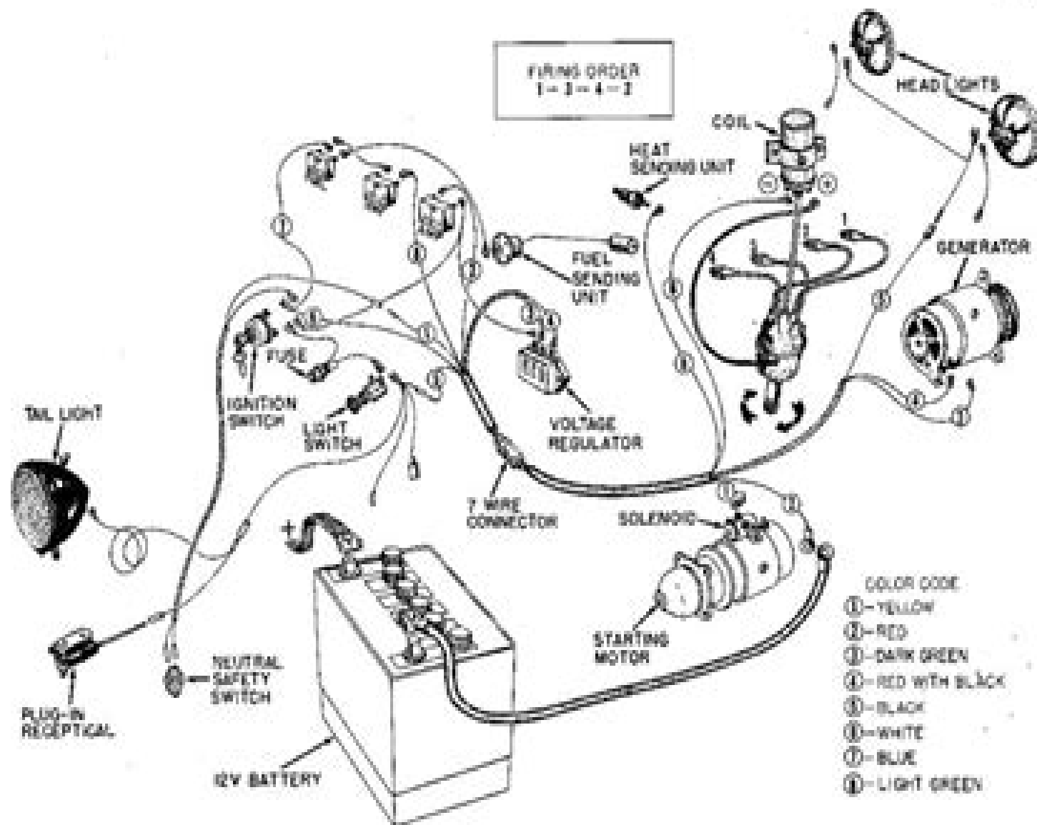
Fig. 108. Case "630" and "630C" Tractors Wiring Diagram
