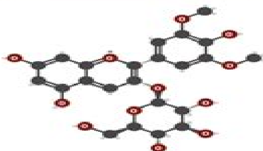
Malvidin 3-glucoside
