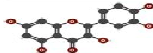
Quercetin
