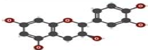
Catechin
