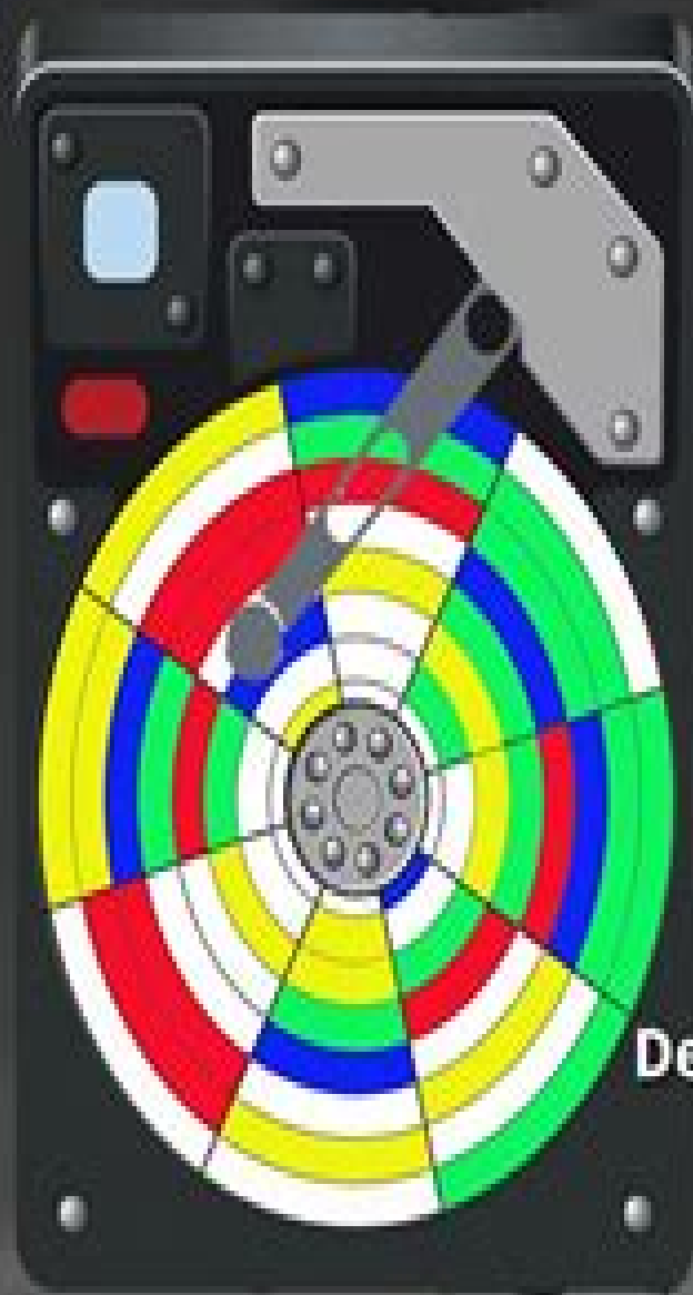
Fragmented disk
