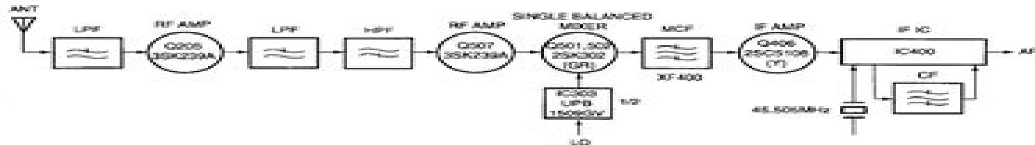
Fig.4 Sub VHF Receiver circuit
