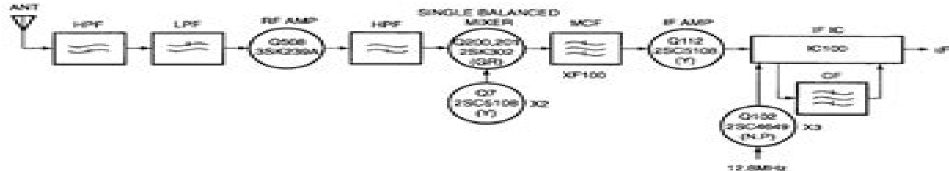
Fig.5 Sub UHF Receiver circuit
