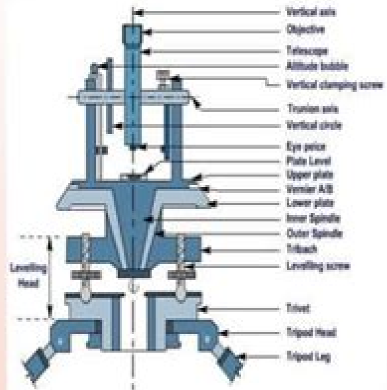
Figure 25.4 Sectional view of a Theodolite
