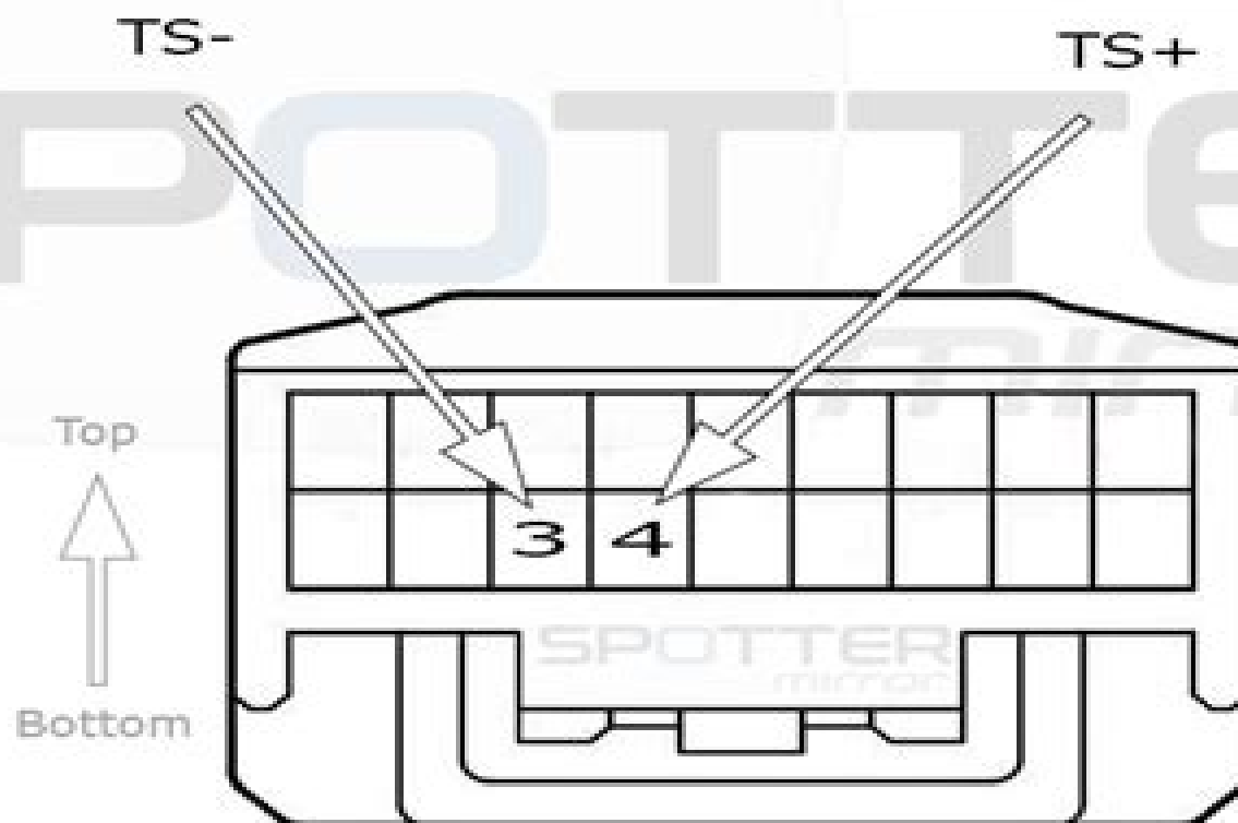
View of connector going to mirror housing
