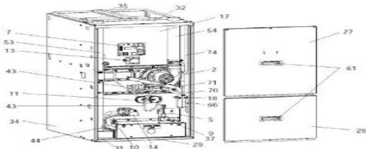
Figure 1: DOWNFLOW/HORIZONTAL NATURAL GAS FURNACES (92%)
