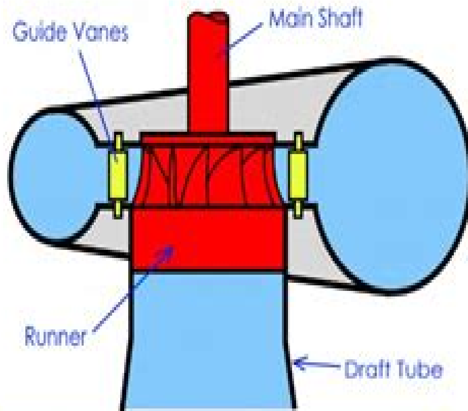
Francis Turbine
