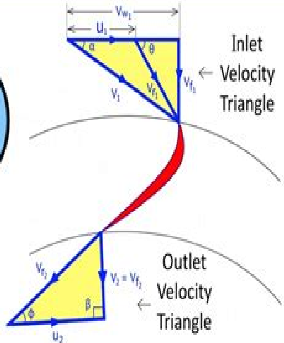
Francis Turbine
