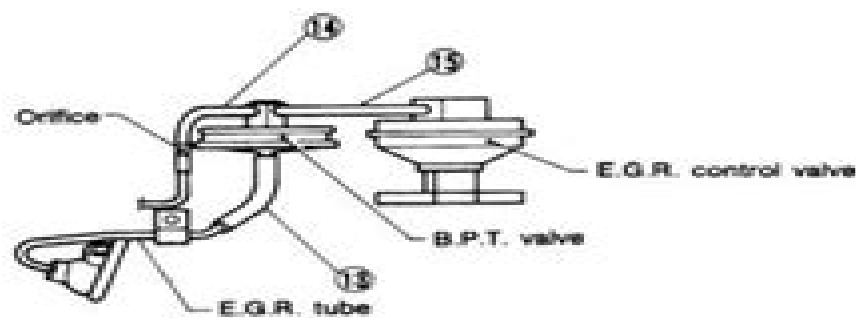
VIEW B
