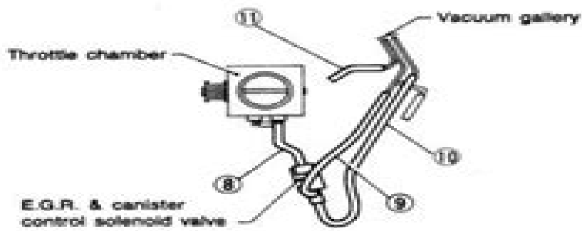
VIEW A
