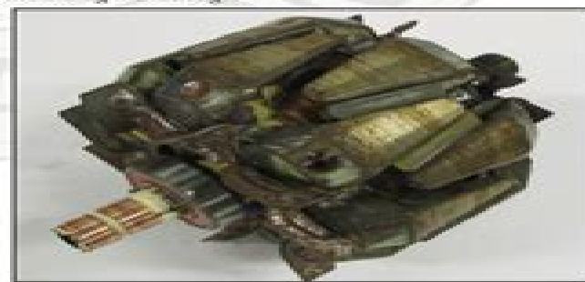
Figure 4 – This Valeo rotor has eight permanent magnets that are spaced in four evenly spaced locations around the rotor.
