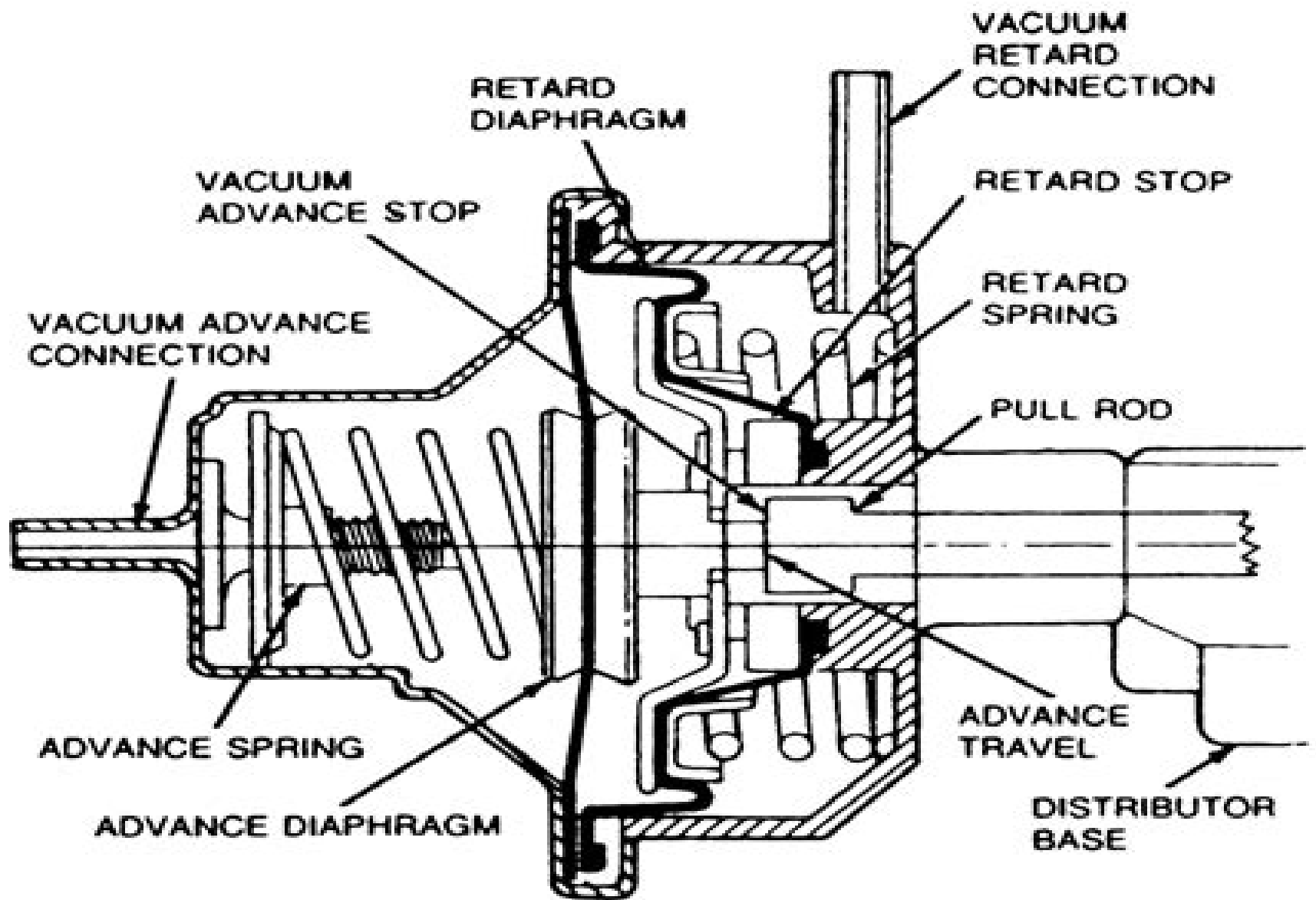
VACUUM ADVANCE AND RETARD DIAPHRAGMS AT REST
