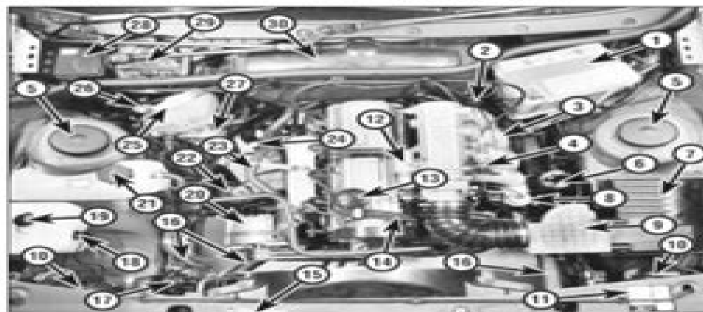
Under-bonnet view of a 2.0 litre DOHC Granada with fuel-injection
