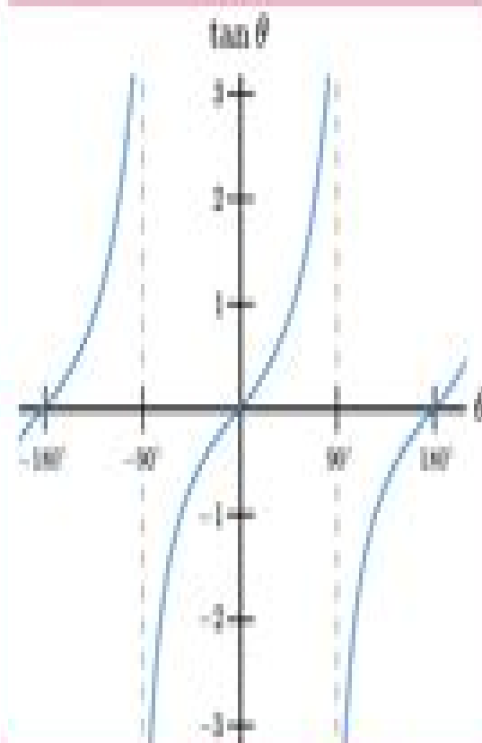
The graph of \tan \theta (the tangent function)
