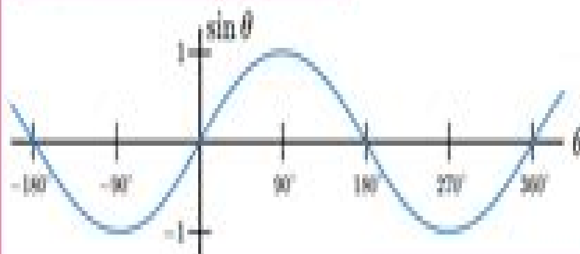
The graph of \sin \theta (the sine function)
