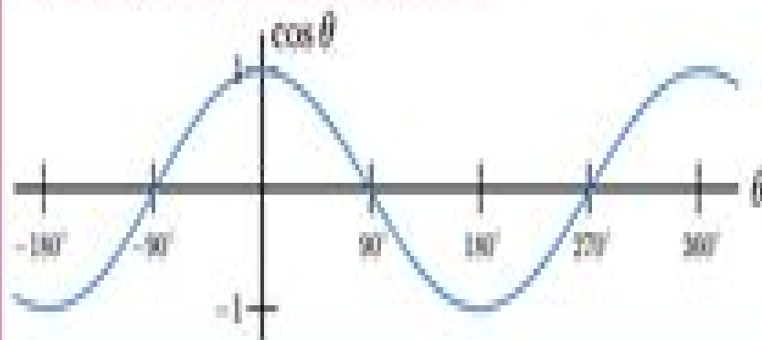
The graph of \cos \theta (the cosine function)
