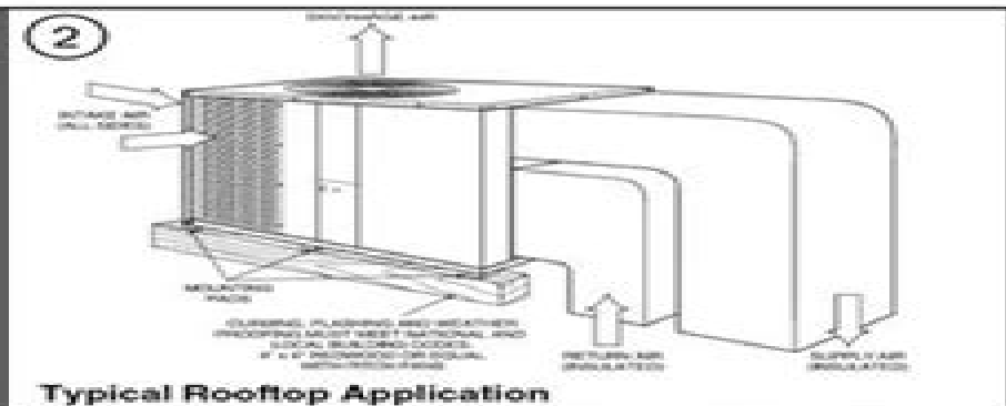
Typical Rooftop Application
