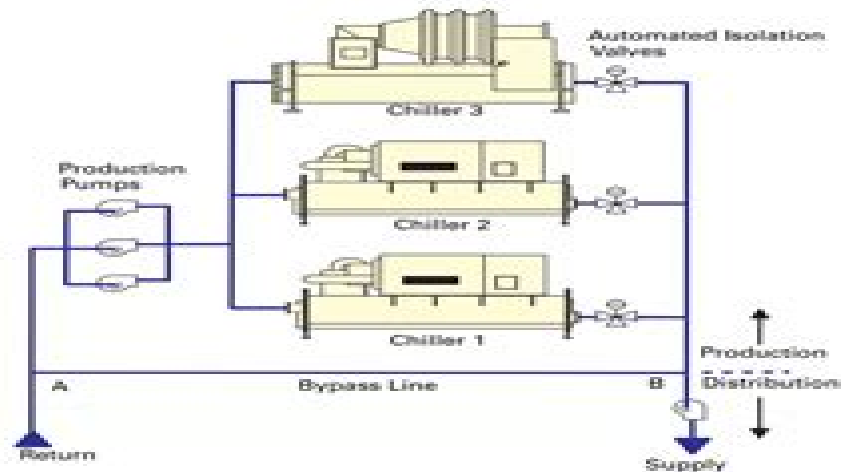
Figure 12: Production loop
