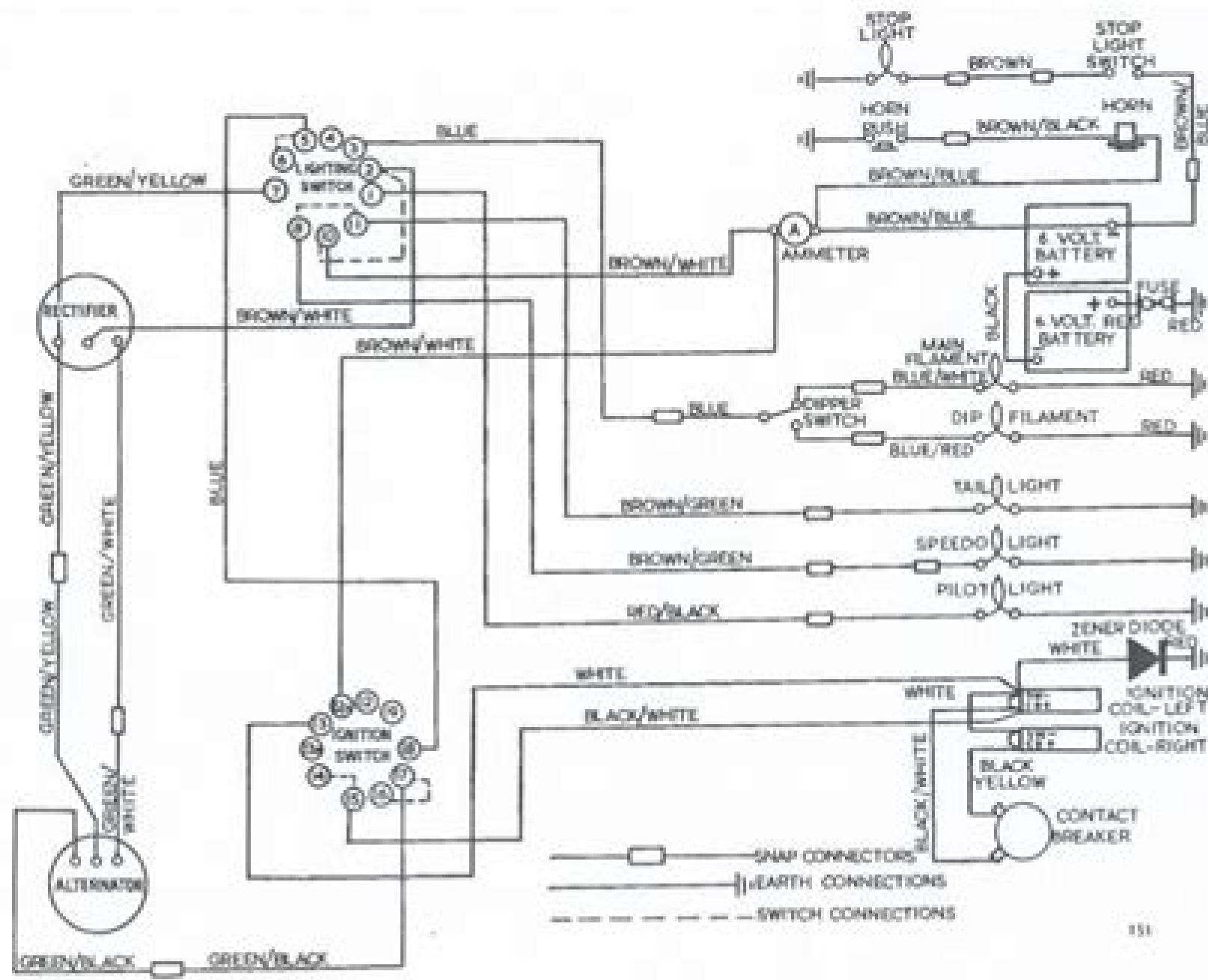
Fig. 147. Wiring diagram—Coil ignition IVT models with Zener Diode and I rate charge control Before engine number DU.34875.
