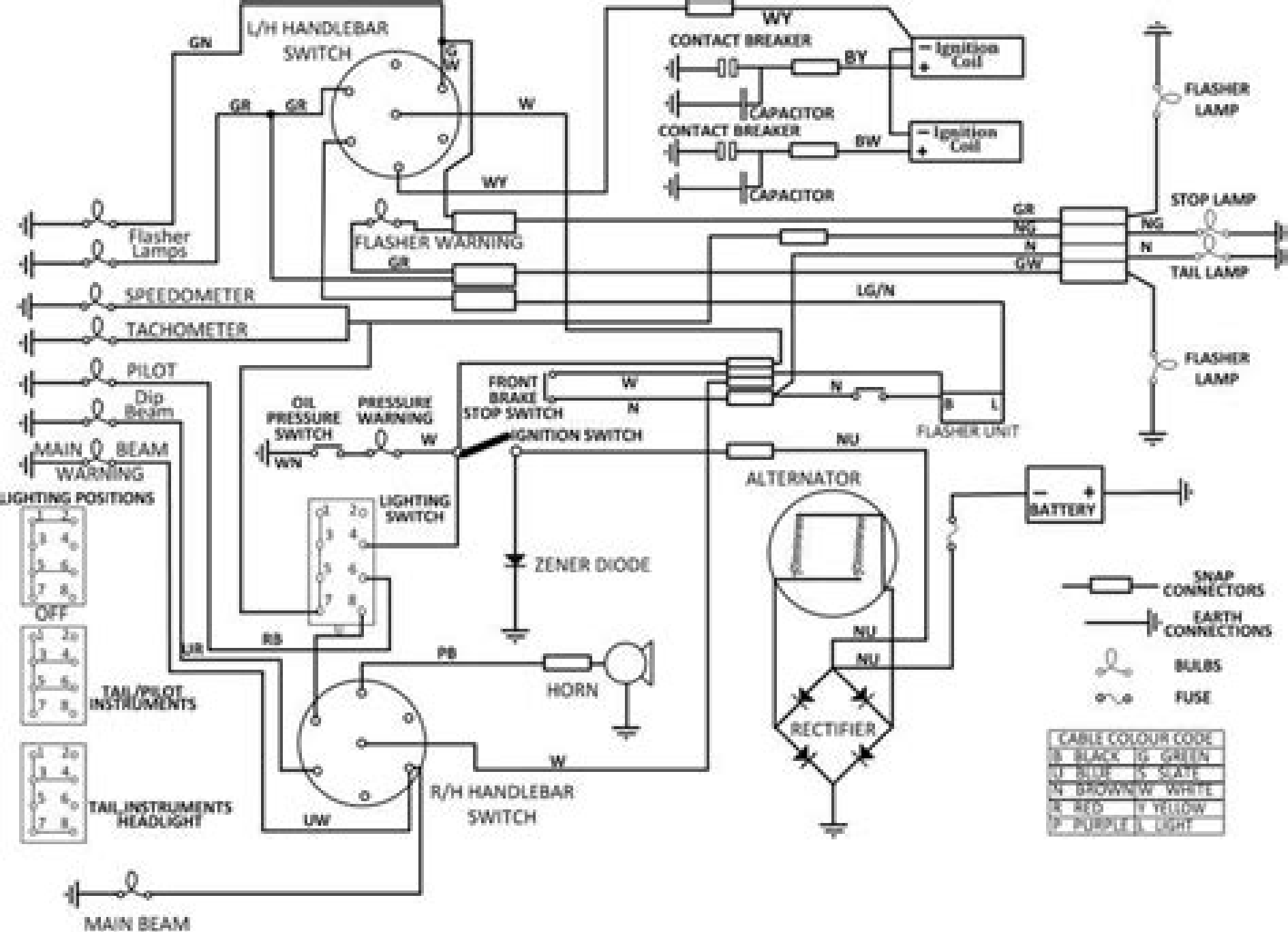
Wiring Diagram (UK & USA) 12 Volt Coil Ignition KE 00001 Onwards
