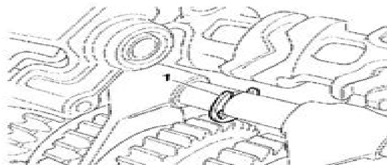
1. E-clip
