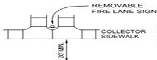
DETAIL 1
