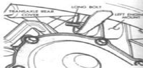
6.22b ... and this long through-bolt
