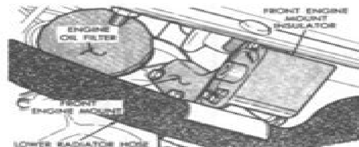
6.20 Remove the front mounting insulator through-bolt and unbolt the insulator from the transaxle
