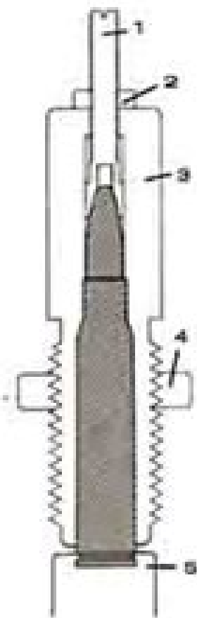
Conway shows progressive steps as the bullet is seated in case.
