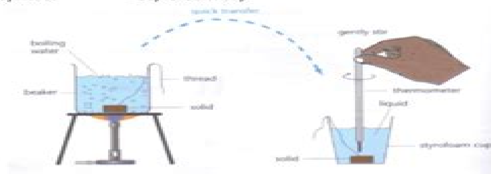
Diagram: Apparatus used for the specific heat capacity of a brass by the method of mixtures
