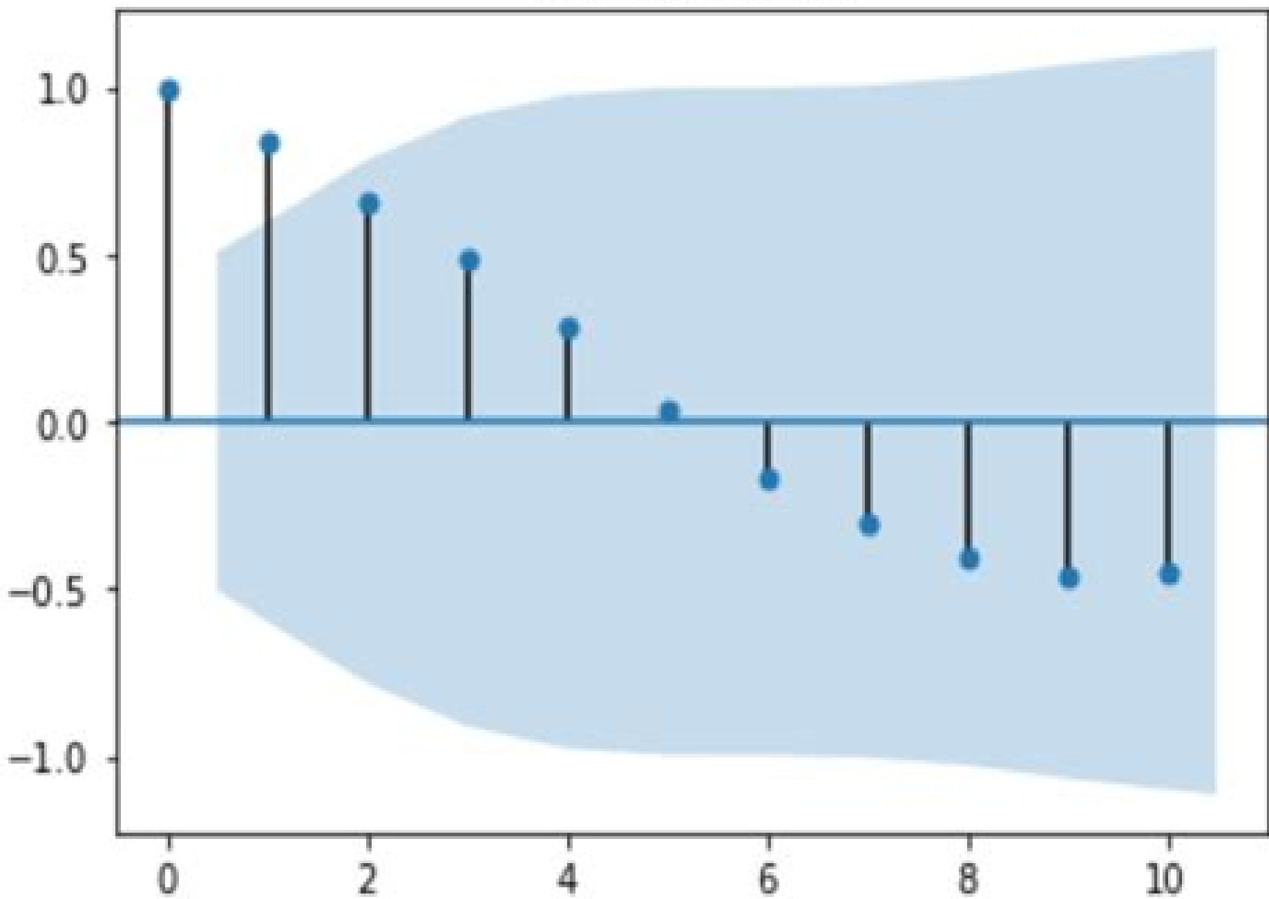
Autocorrelation
