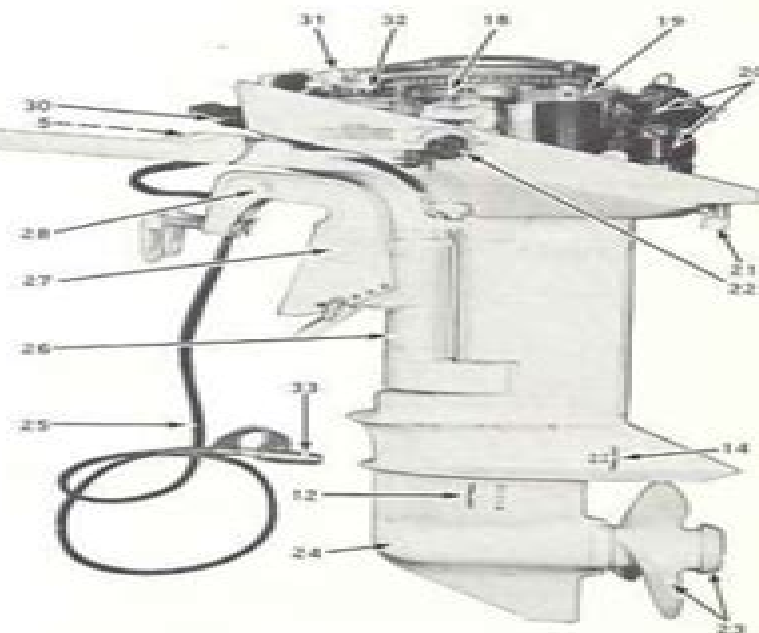
Figure 1-2. Port Side (Electric Start)
