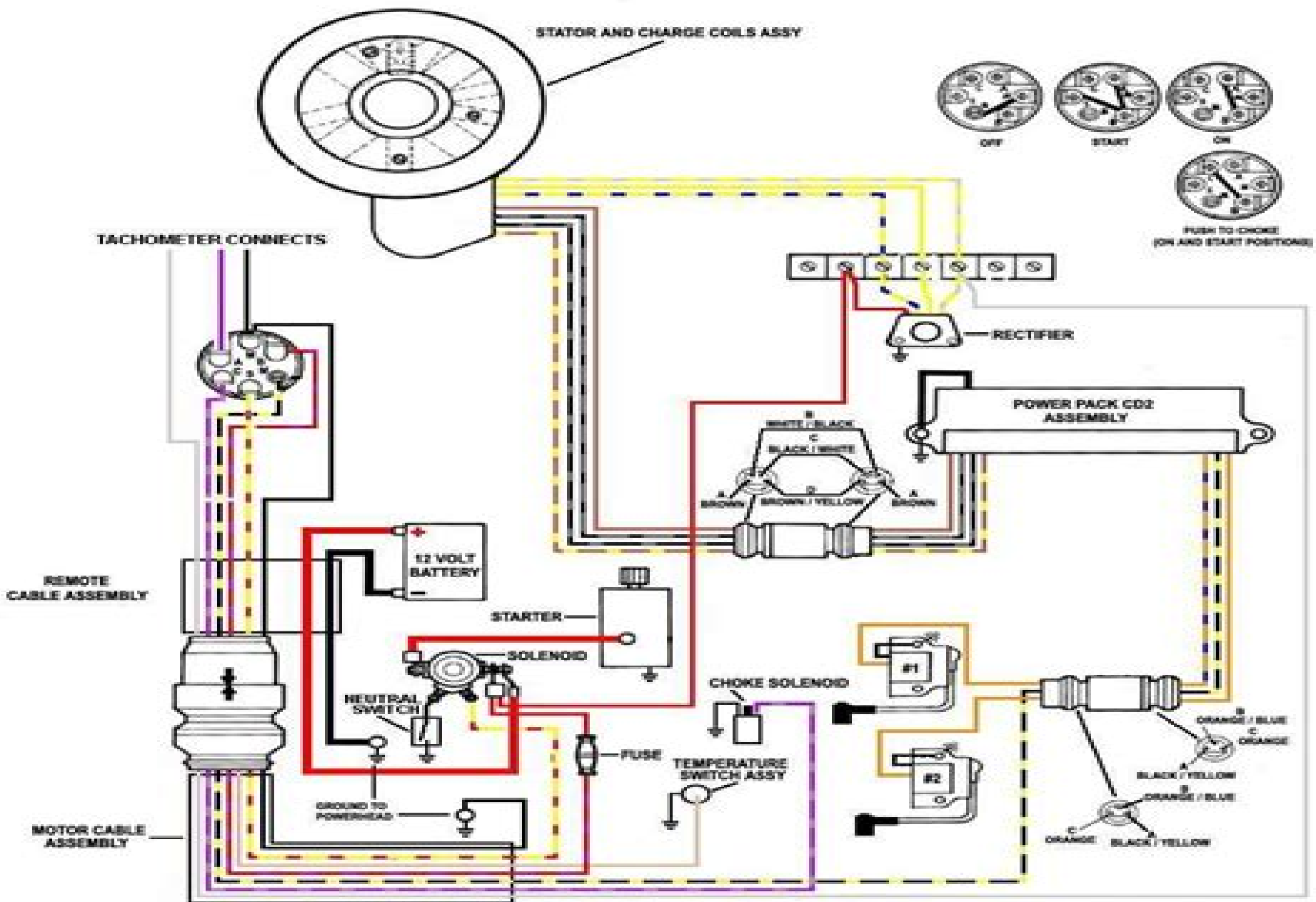
WIRING DIAGRAM
