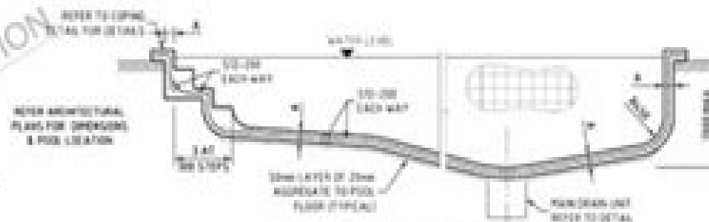
TYPICAL LONGITUDINAL SECTION SCALE 1/4" = 1'-0"
