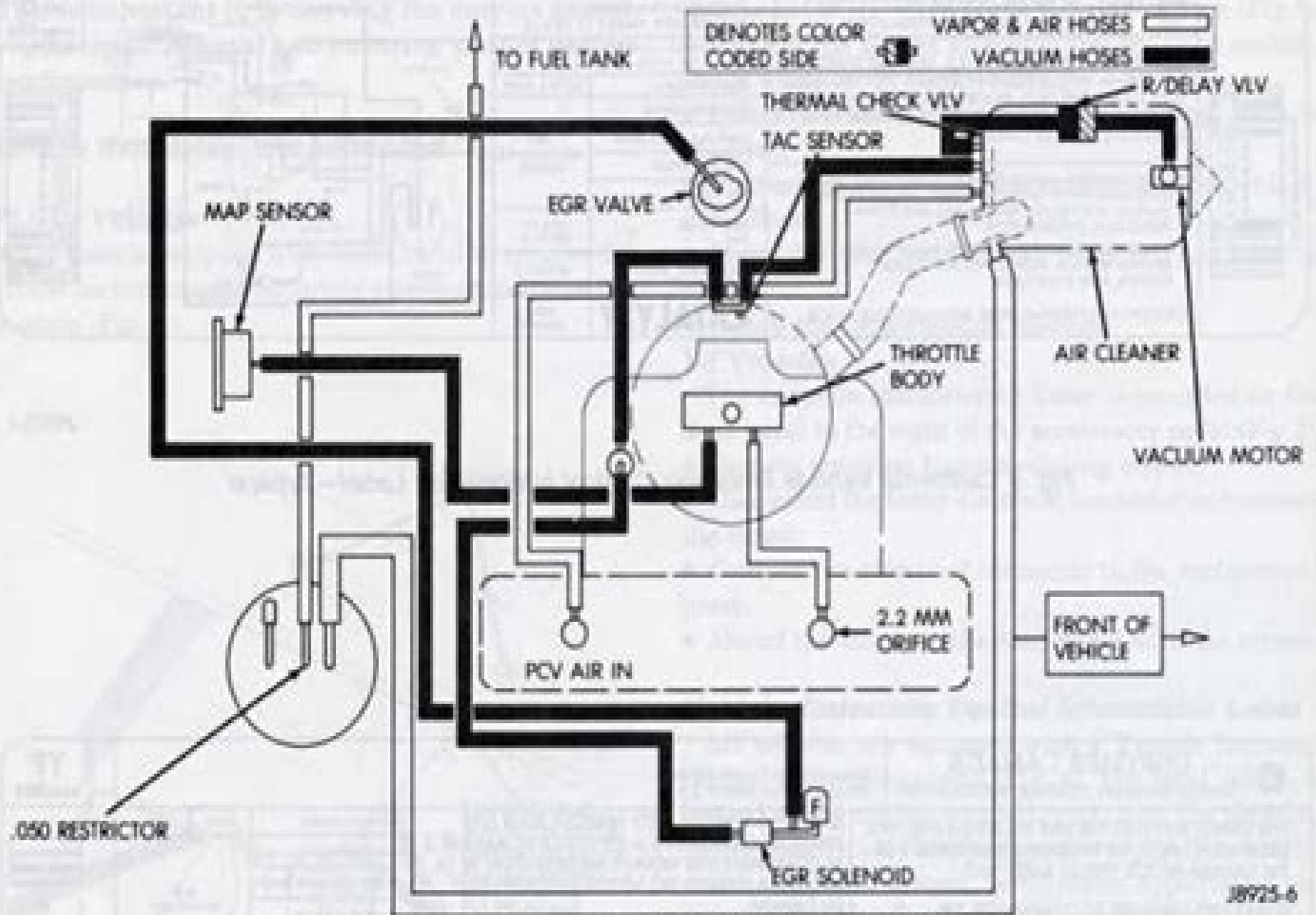
Fig. 7 Emissions Schematic—MJ/XJ Vehicles with 2.5L Engine
