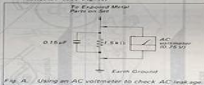
Fig. A. Using an AC voltmeter to check AC leakage.
