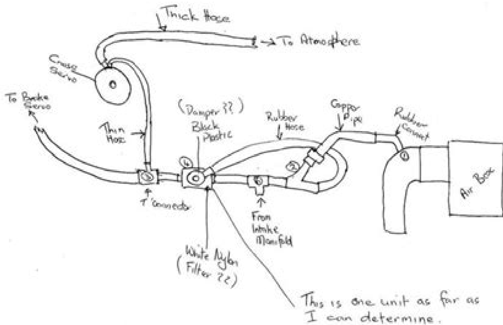
Cruise Control Vacuum Diagram (Sketched from 1985 911 3.2 Japanese Import)
