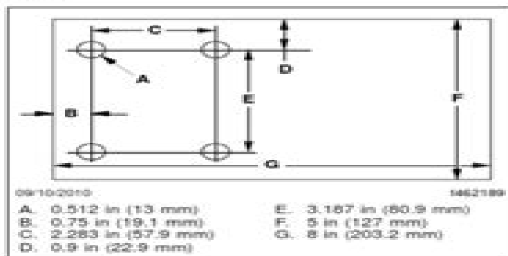
Fig. 1. Holding Fixture Template
