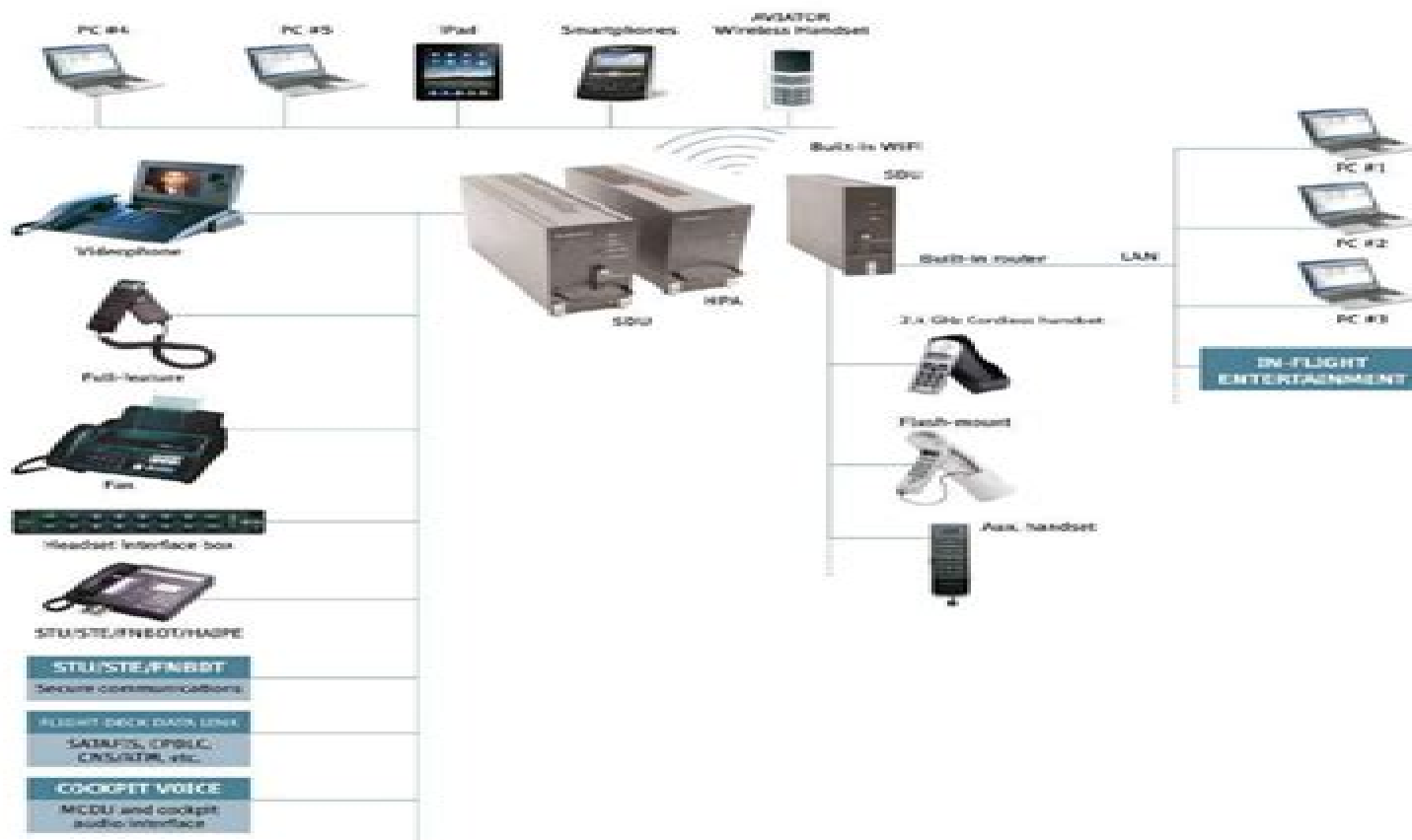
Figure 2-1: Communication devices for the AVIATOR 700 system (example)
