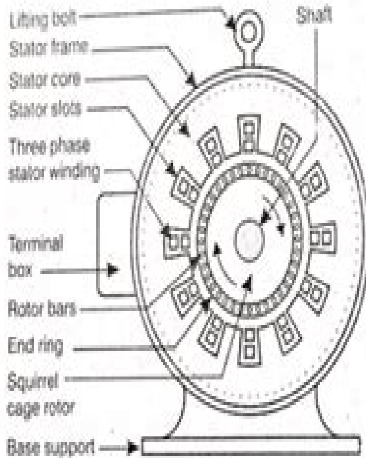
Sectional view
