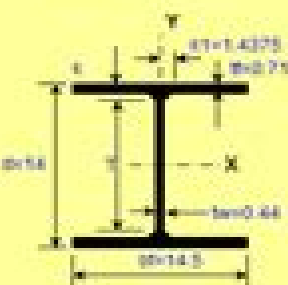
WT, S, M, HP Shapes
