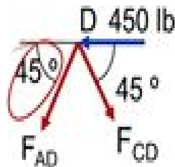
FBD of pin D
