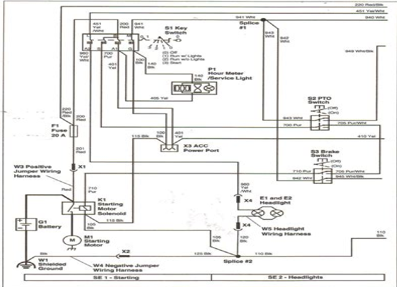
Main Wiring Schematic L100/L110/L120
