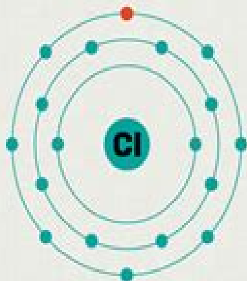
Ionic Bond
