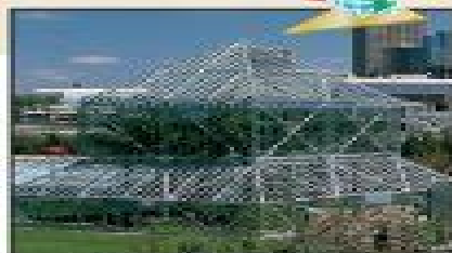
The roof of the Cowles Conservatory in Minneapolis, Minnesota, shows the midsegments of a triangle.
