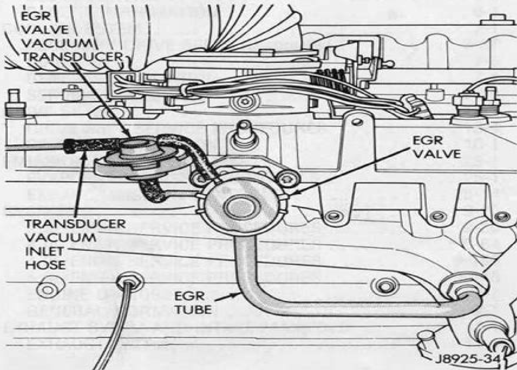
Fig. 48 EGR Valve and Transducer—4.0L Engine
