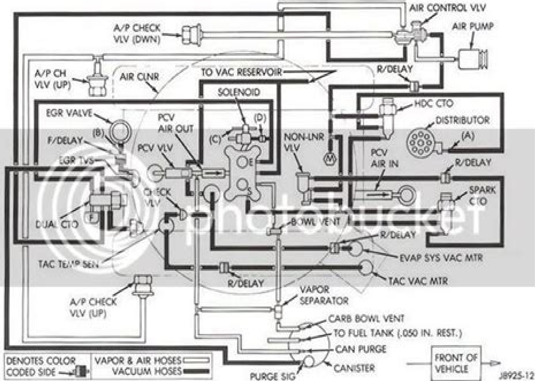
1989 Fig. 13 Emissions Schematic—Model 15 with 5.9L Engine and Heavy Duty Cooling
