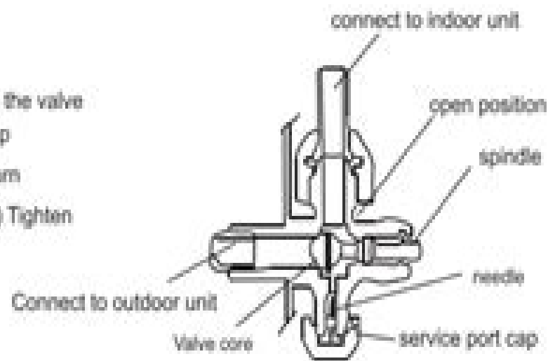
3-way valve diagram
