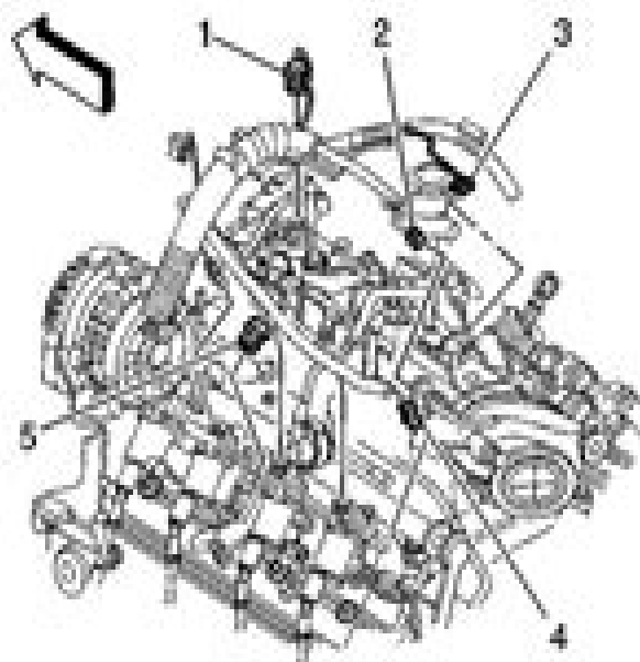
Fig. 54: View Of Top Of Engine Wiring Harness Courtesy of GENERAL MOTORS CORP.
