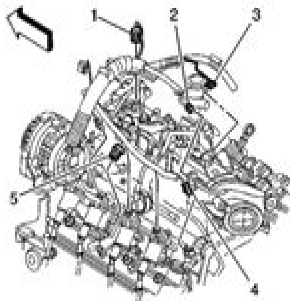
Fig. 55: View Of Top Of Engine Wiring Harness Courtesy of GENERAL MOTORS CORP.
